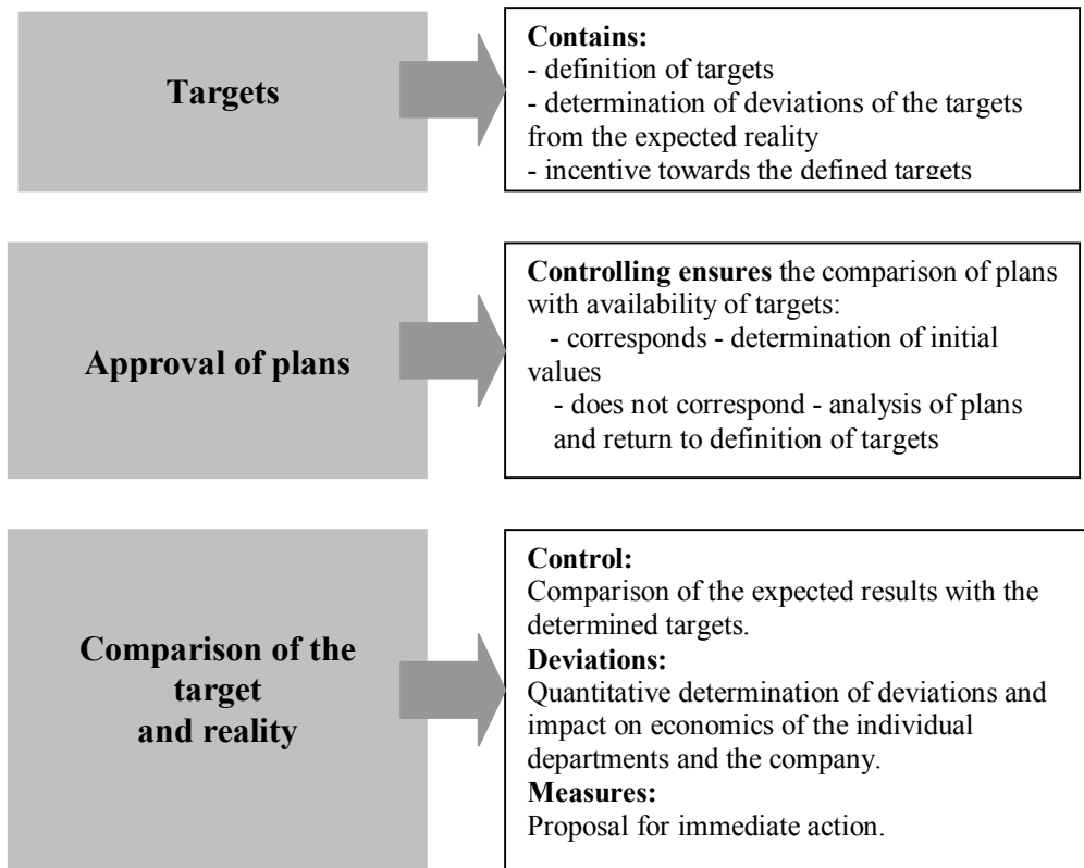
Figure 2. Operational controlling
